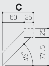
SUPPORTI INCLINATI SLANTED SUPPORTS
