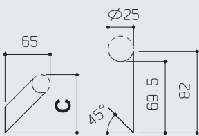
SUPPORTI INCLINATI SLANTED SUPPORTS
