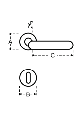
Maniglia con rosetta e bocchetta Handle with rose and lock profile
