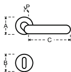
Maniglia con rosetta e bocchetta Handle with rose and lock profile
